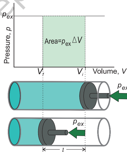
Fig. 5.5 (a) Work done on an ideal gas in a cylinder when it is compressed by a constant external pressure, p_{\text{ex}} (in single step) is equal to the shaded area.
